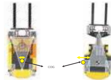
Counterbalance Forklift
